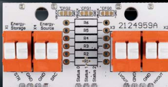
Universelles Energy-Harvesting-Modul
